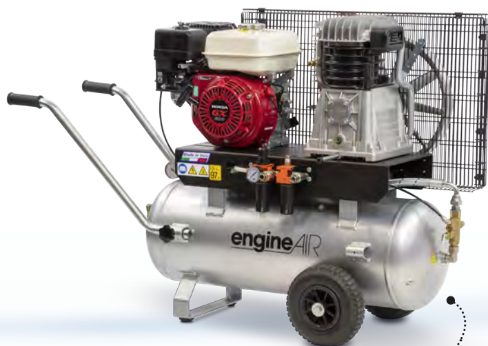
engineAIR 6/50 10 Petrol 5,8 hp, 50 litros, 10 bar
